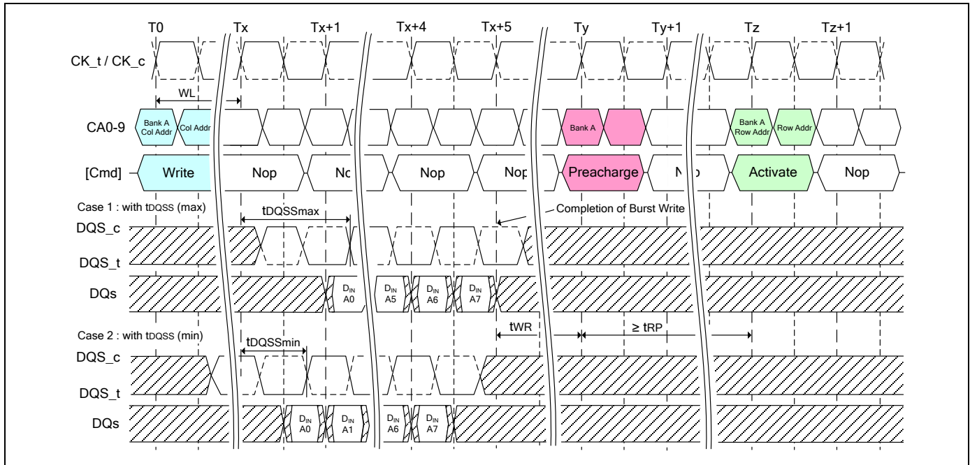
Figure 23 - Burst Write Followed by Precharge
