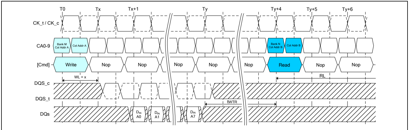
Figure 19 - Burst Write Followed By Burst Read
