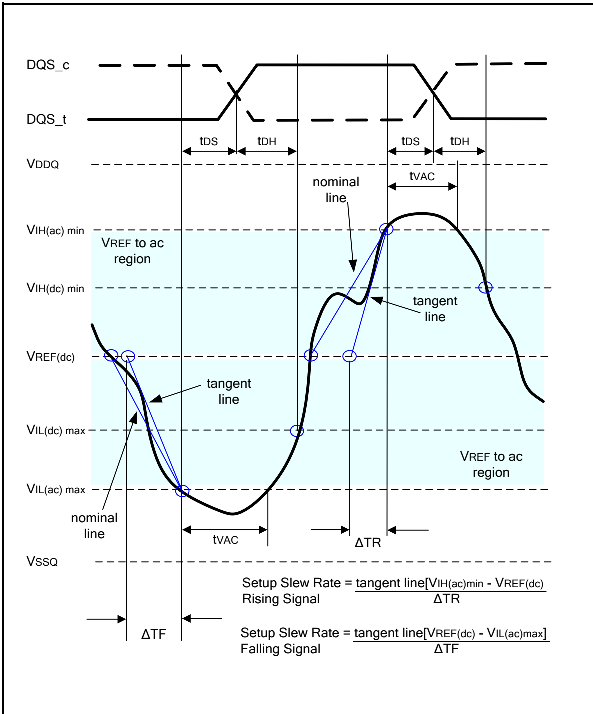
Figure 82 - Tangent line for setup time t_{DS} for DQ with respect to strobe
