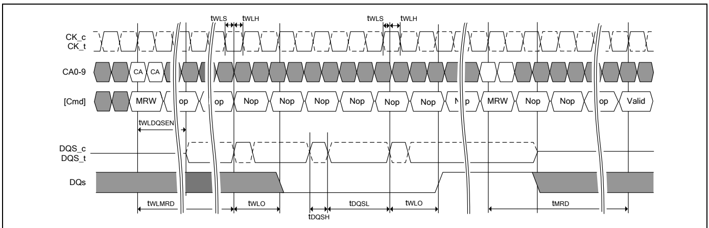
Figure 44 - Write Leveling Timing
