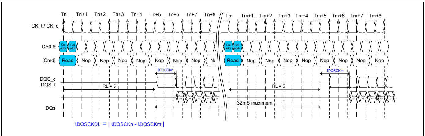
Figure 10 - t_{DQSKDL} timing
