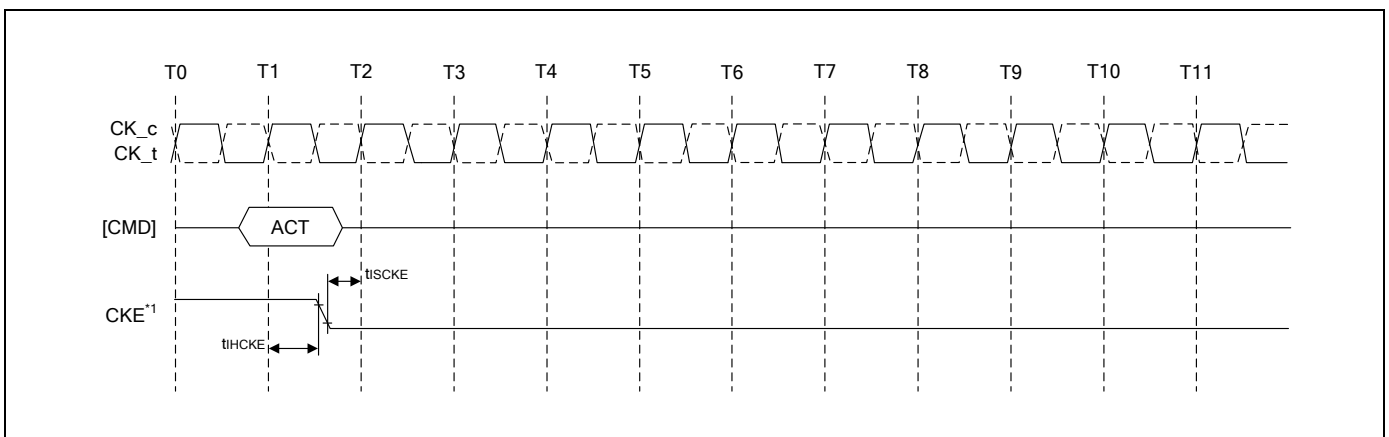
Figure 57 - Activate Command to Power-Down Entry
