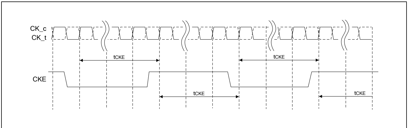
Figure 50 - CKE-Intensive Environment
