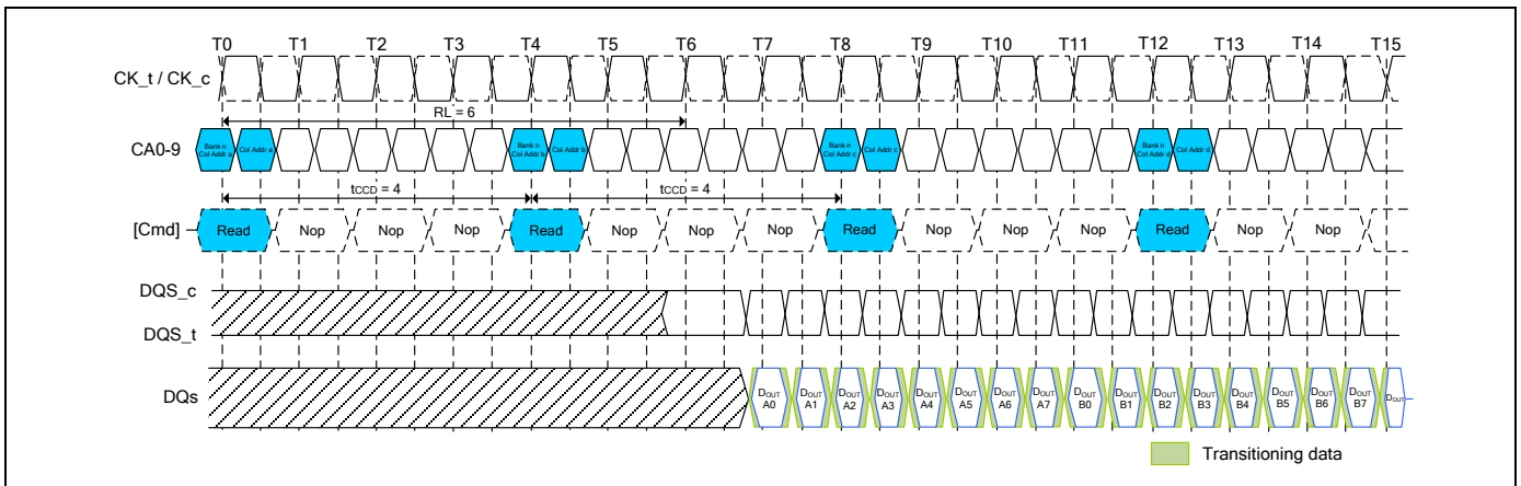
Figure 14 - Seamless Burst Read
