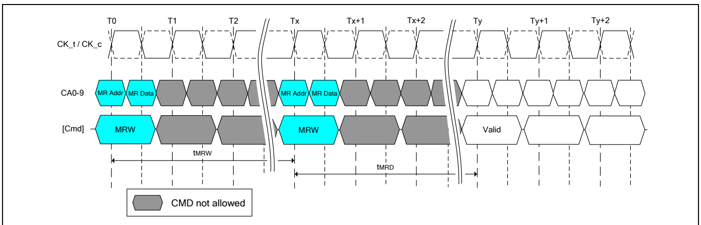
Figure 37 - Mode Register Write Timing
