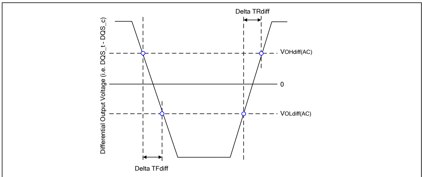
Figure 69 - Differential Output Slew Rate Definition
