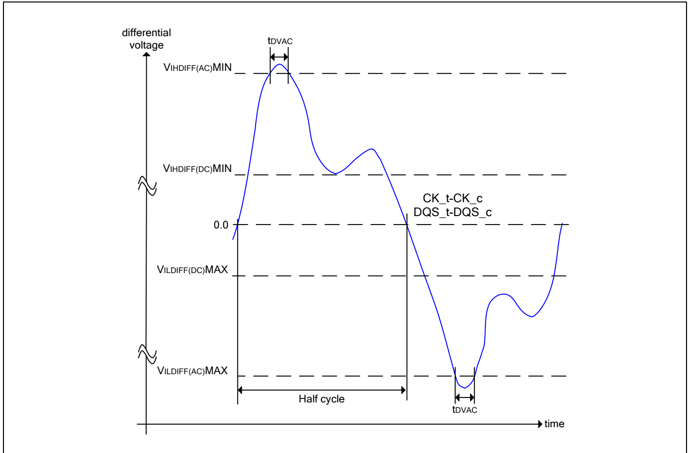
Figure 64 - Definition of Differential ac-swing and “time above ac-level” tDVAC
