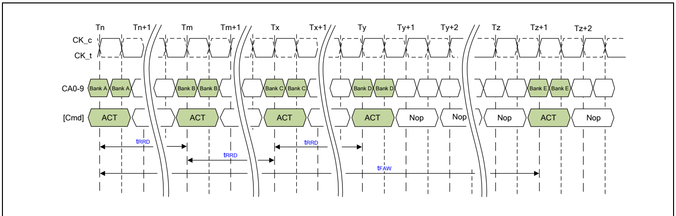
Figure 4 - tFAW Timing
