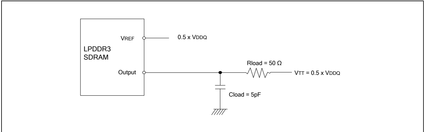
Figure 71 - HSUL_12 Driver Output Reference Load for Timing and Slew Rate
