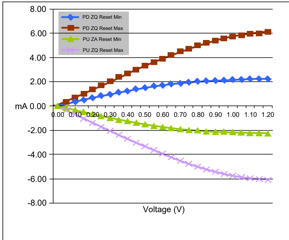
Figure 73 - I-V Curve after ZQ Reset
