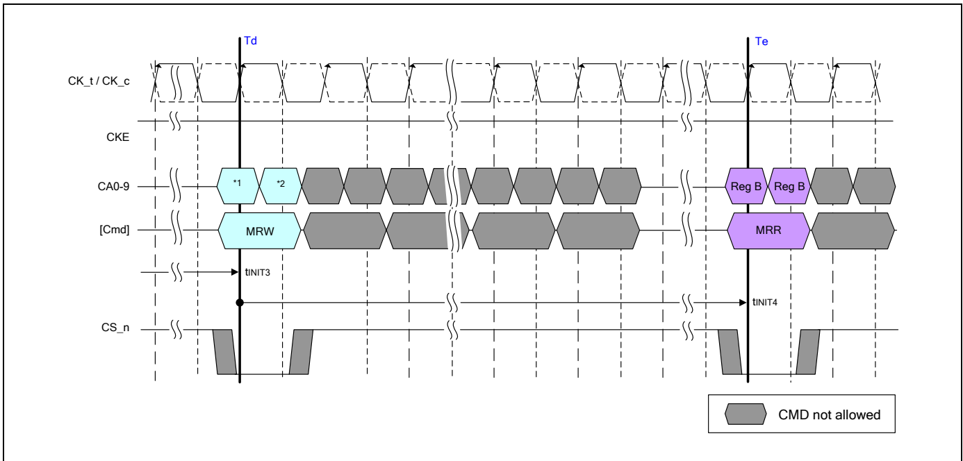
Figure 38 - Mode Register Write Timing for MRW RESET
