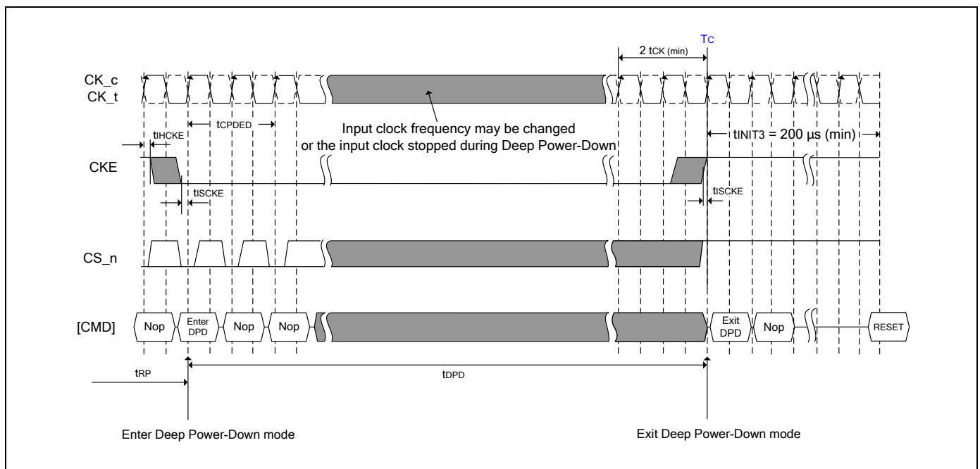
Figure 61 - Deep power down entry and exit timing diagram
