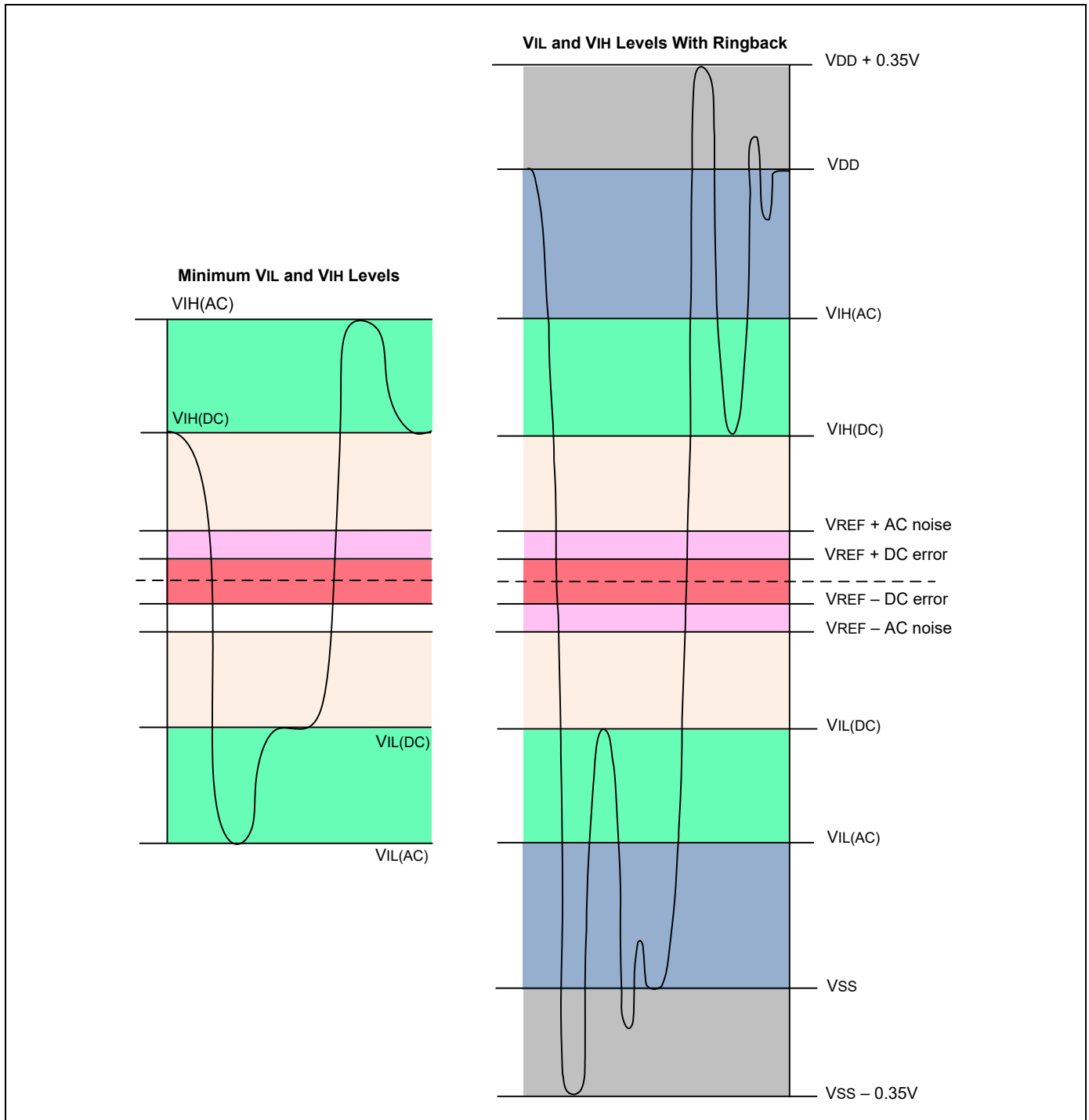
Figure 63 - LPDDR3 Input Signal
