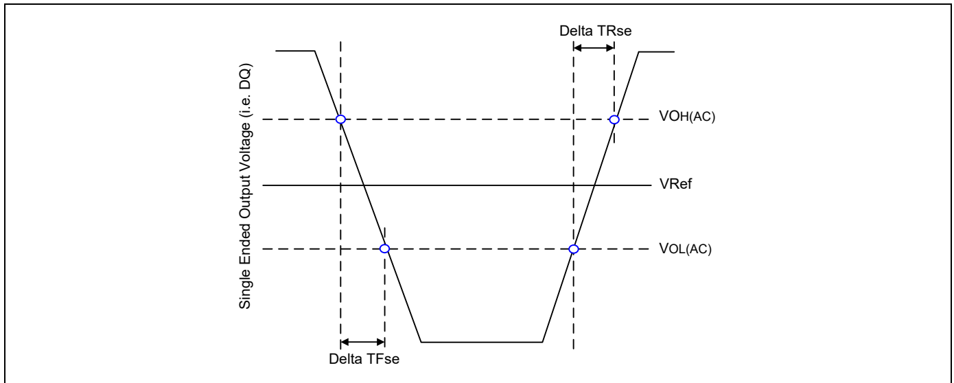
Figure 68 - Single Ended Output Slew Rate Definition
