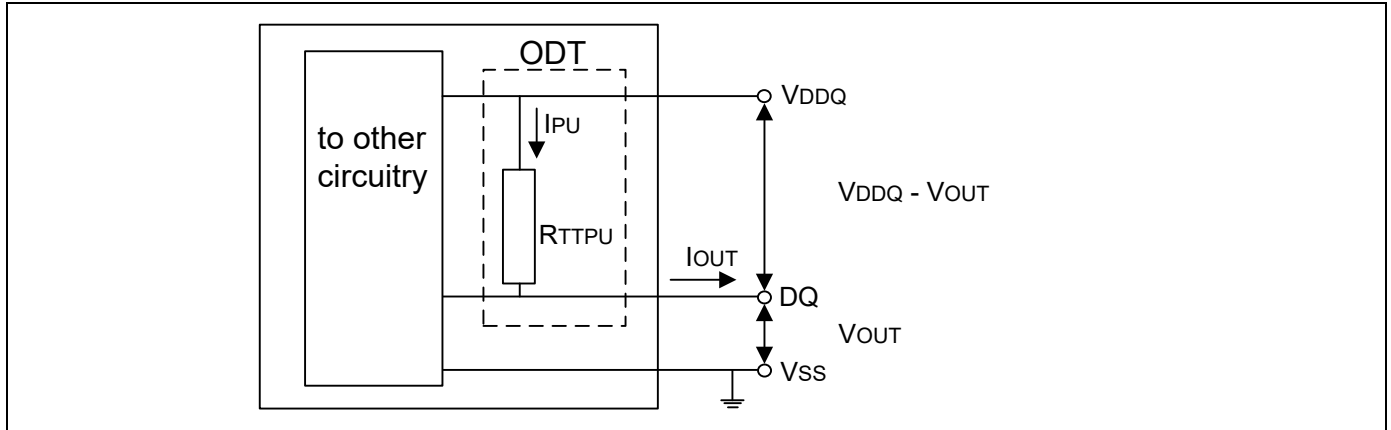
Figure 75 - Functional representation of On-Die Termination
