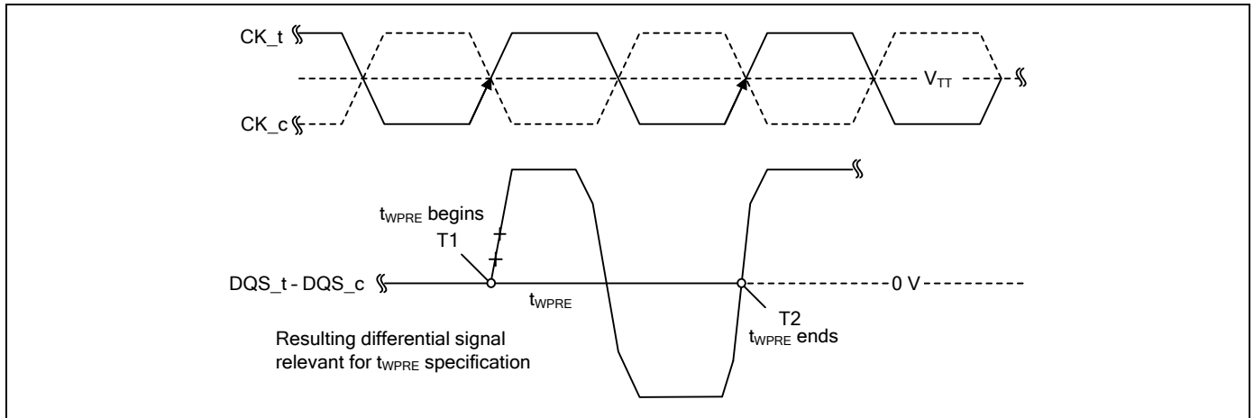
Figure 17 - Method for calculating t_{WPRE} Transitions and Endpoints
