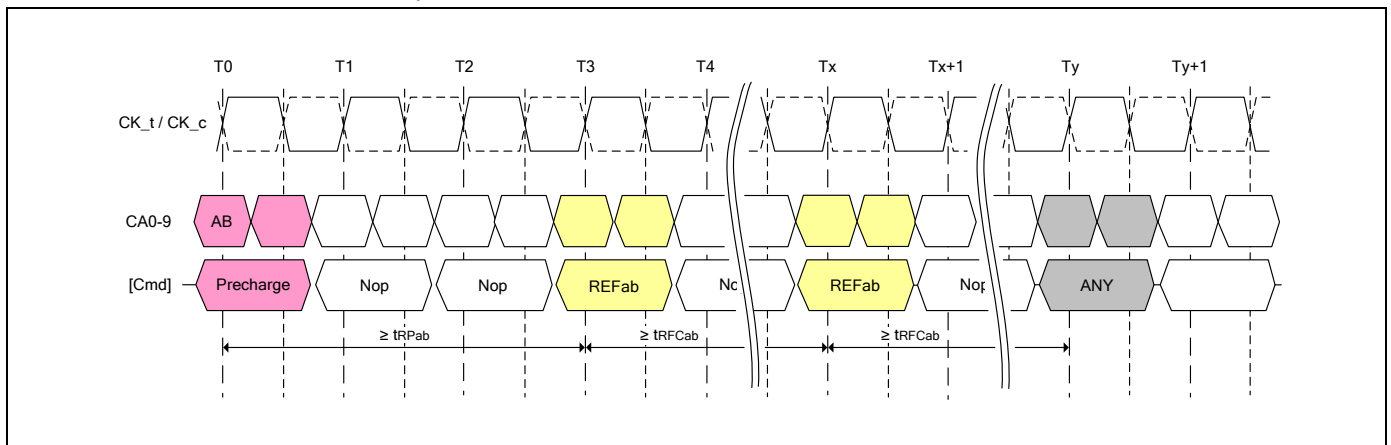
Figure 29 - All-Bank Refresh Operation
