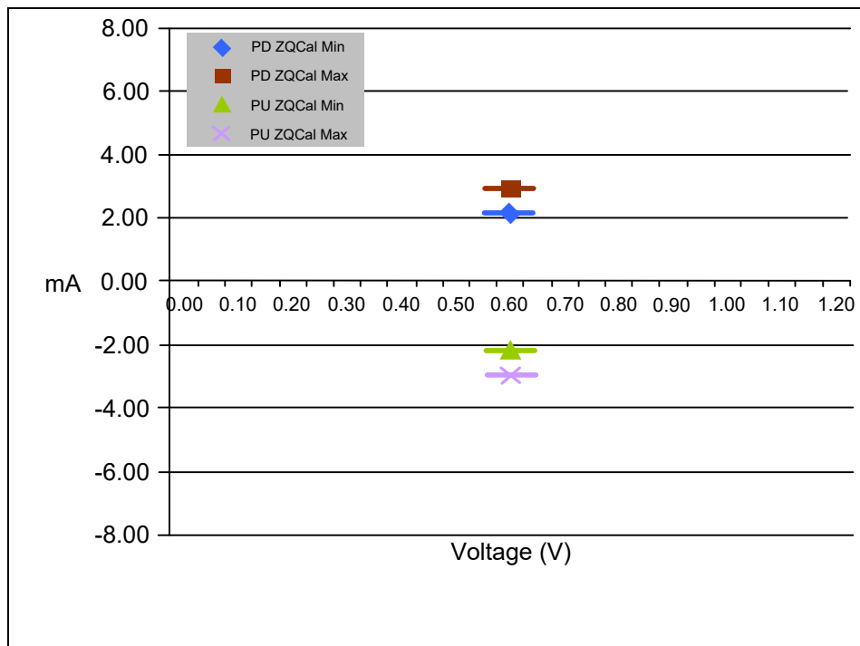
Figure 74 - I-V Curve after Calibration
