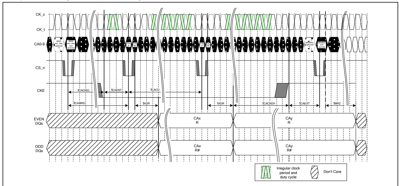
Figure 43 - CA Training Timing Chart
