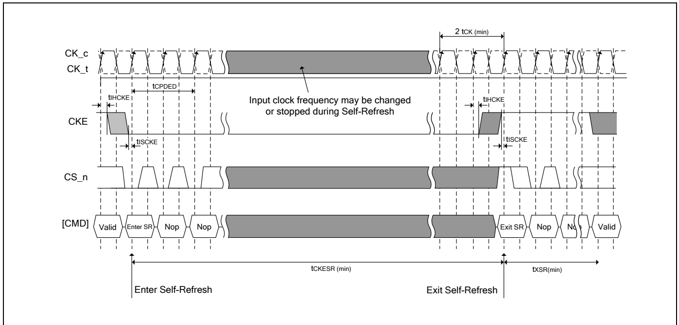
Figure 30 - Self-Refresh Operation
