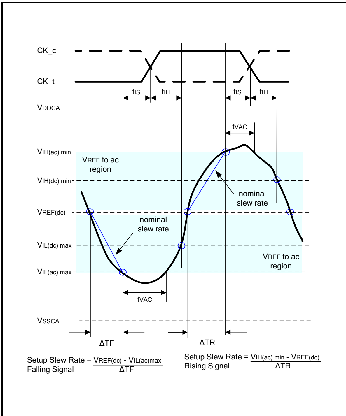
Figure 76 - Nominal slew rate and t_{VAC} for setup time t_{IS} for CA and CS n with respect to clock
