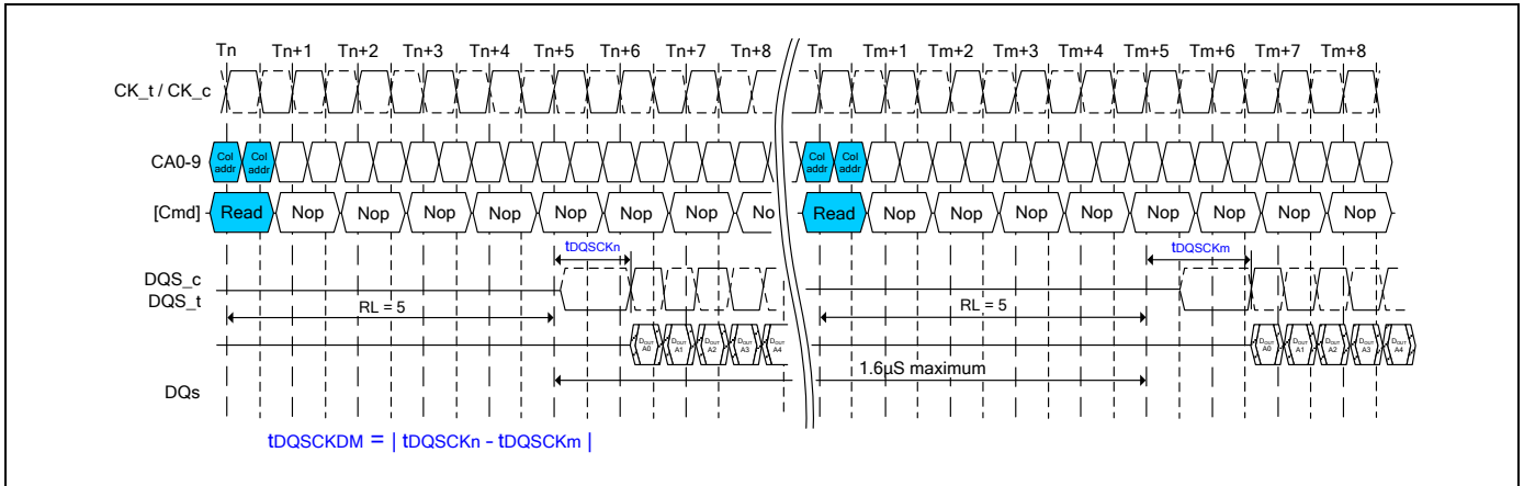
Figure 11 - tDQCKDM timing
