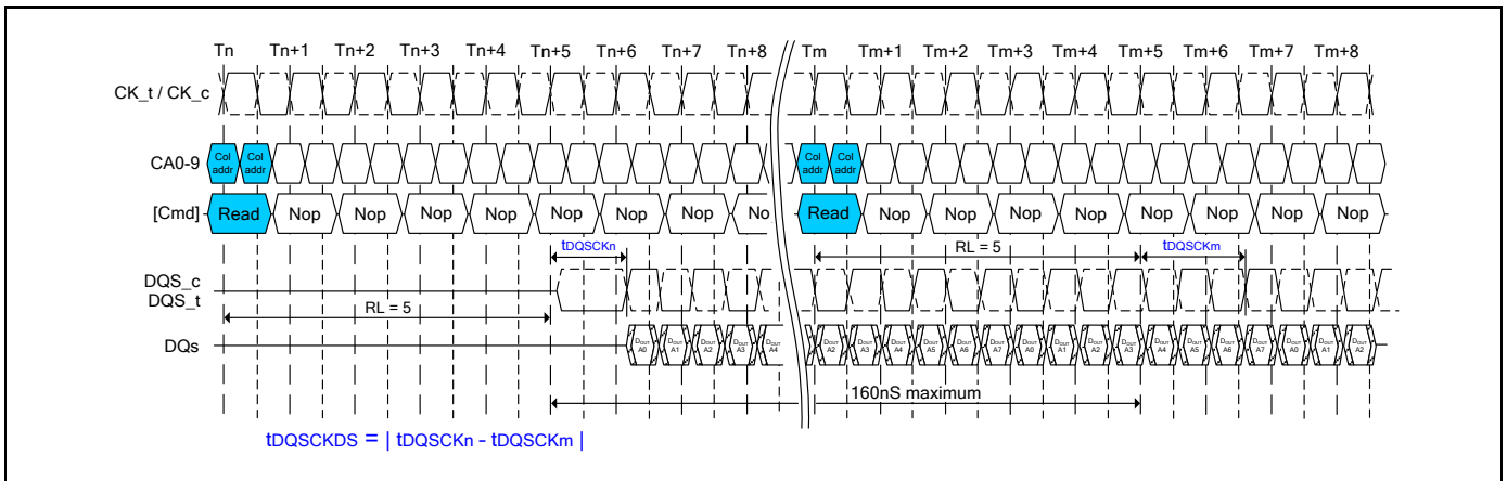
Figure 12 - tDQCKDS timing
