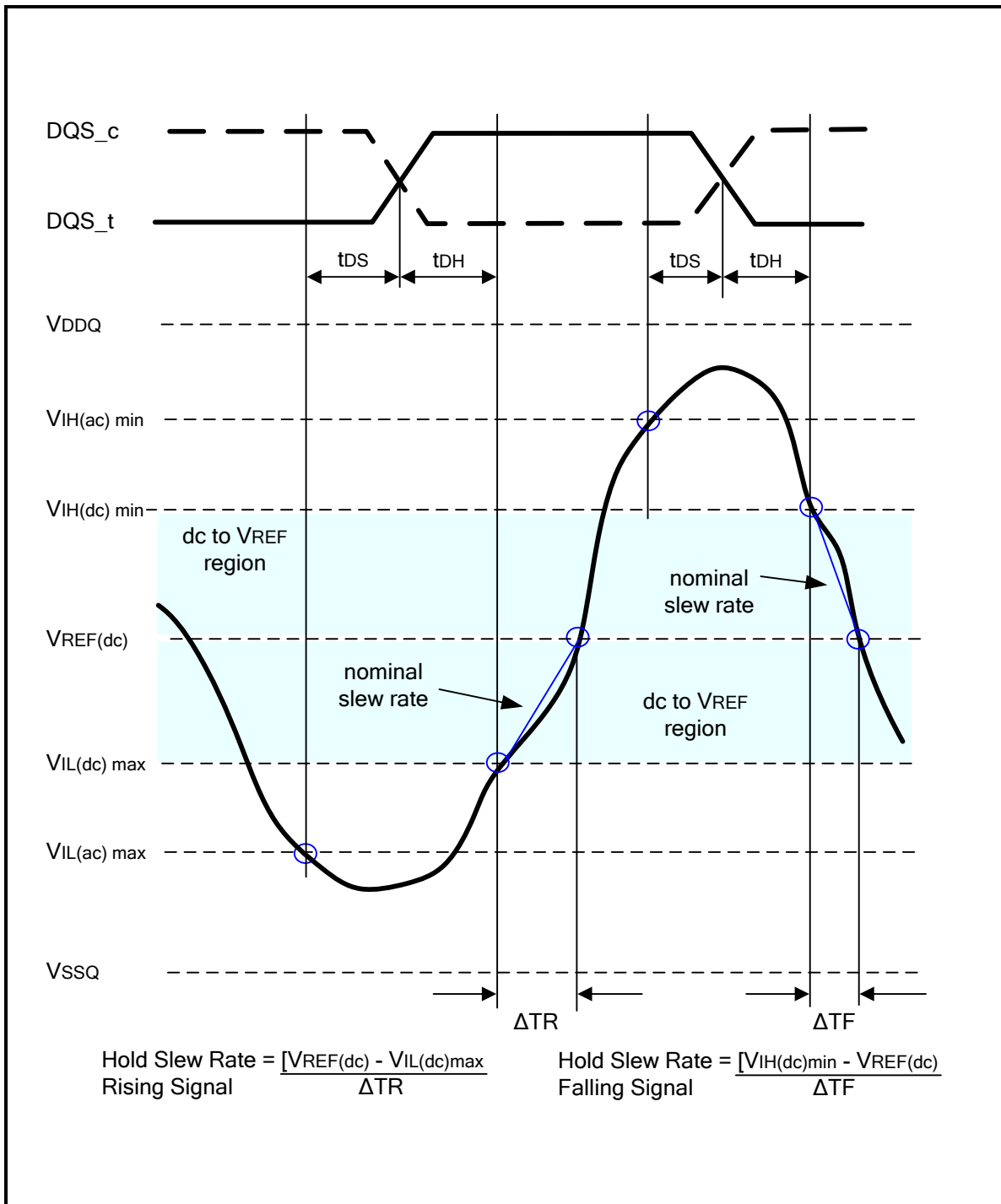
Figure 81 - Nominal slew rate for hold time t_{DH} for DQ with respect to strobe
