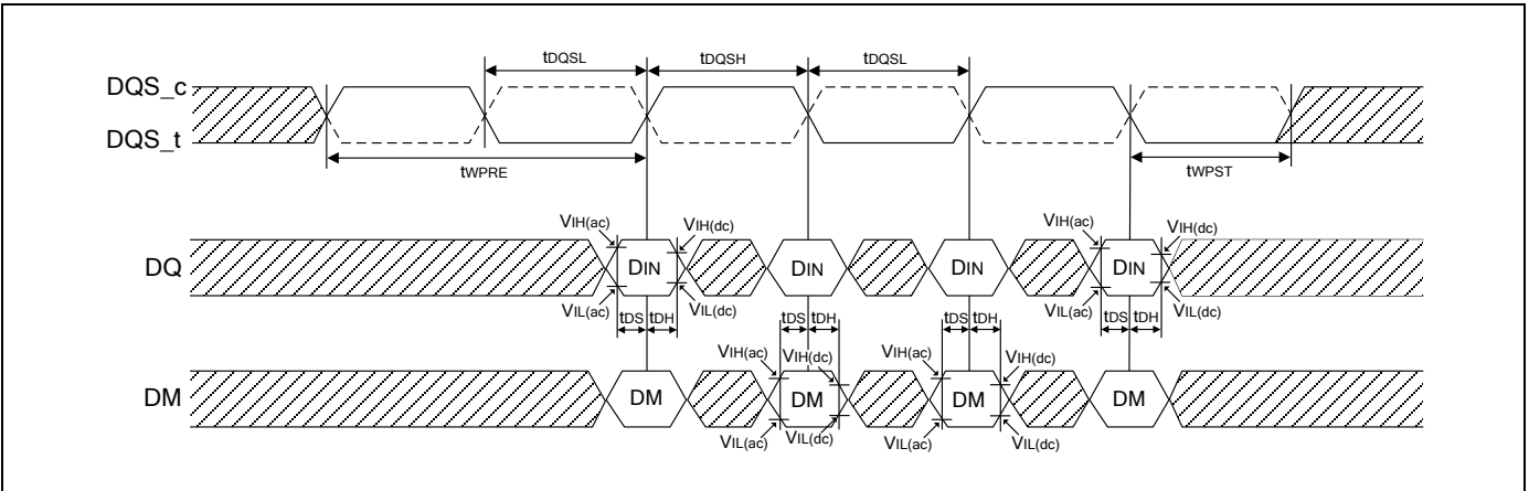
Figure 15 - Data input (write) timing
