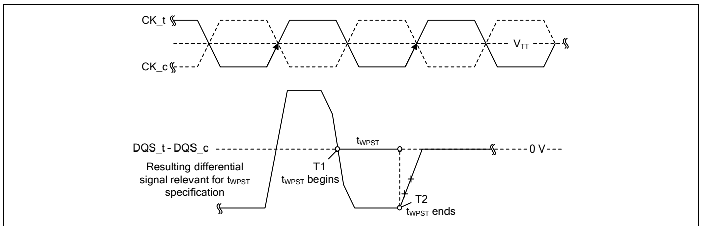
Figure 18 - Method for calculating t_{WPST} Transitions and Endpoints
