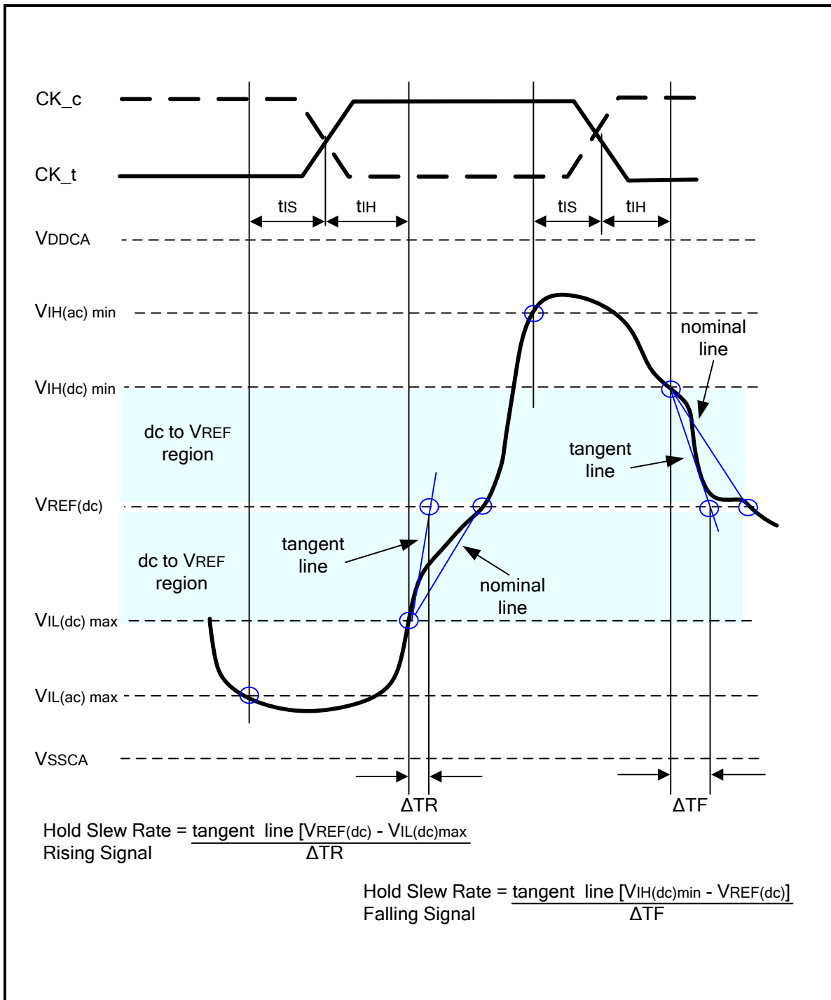
Figure 79 - Tangent line for hold time t IH for CA and CS n with respect to clock
