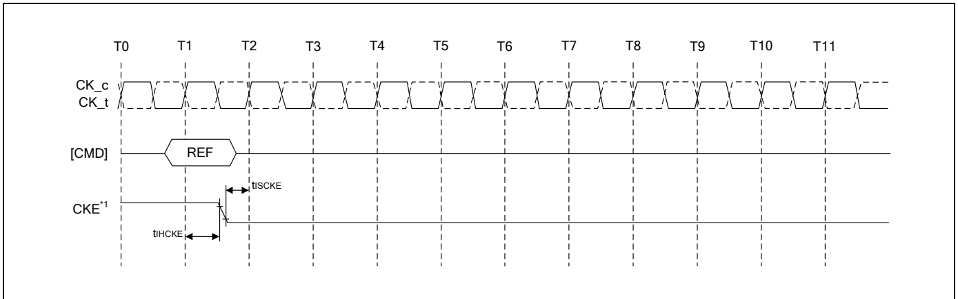
Figure 56 - Refresh Command to Power-Down Entry
