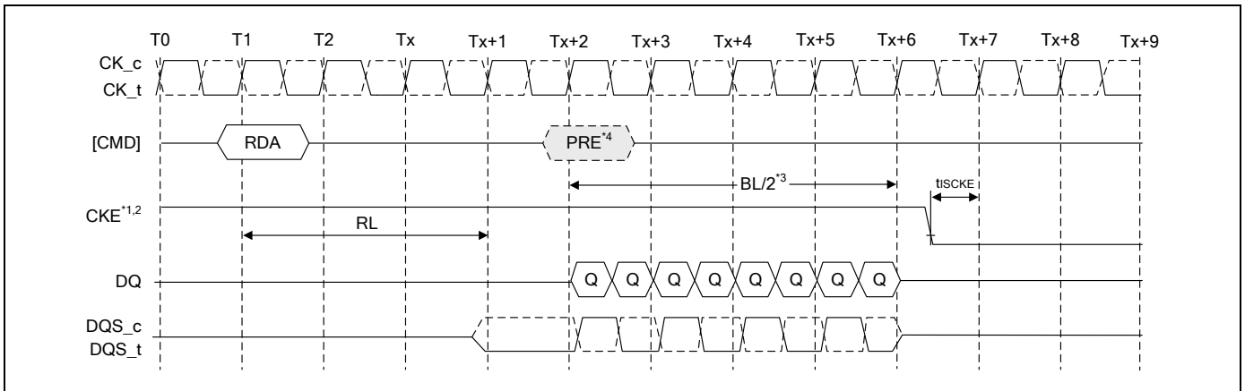
Figure 53 - Read with Auto Precharge to Power-Down Entry
