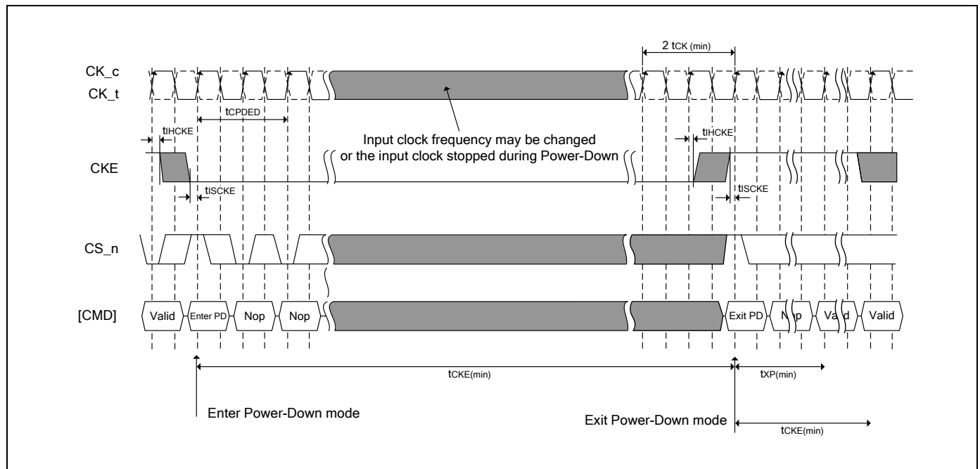
Figure 49 - Basic Power-Down Entry and Exit Timing
