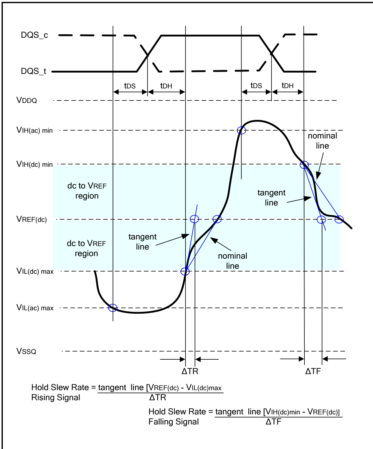
Figure 83 - Tangent line for hold time t_{DH} for DQ with respect to strobe
