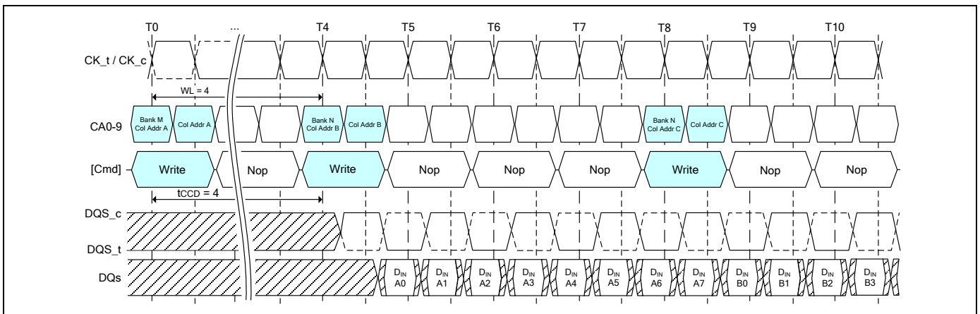
Figure 20 - Seamless burst write: WL = 4, tCCD = 4
