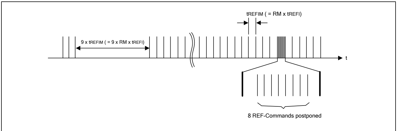
Figure 27 - Postponing Refresh Commands
