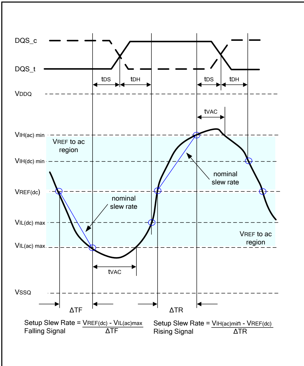
Figure 80 - Nominal slew rate and t_{VAC} for setup time t_{DS} for DQ with respect to strobe
