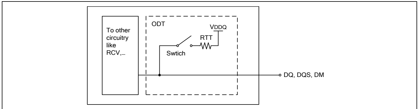
Figure 45 - Functional Representation of ODT
