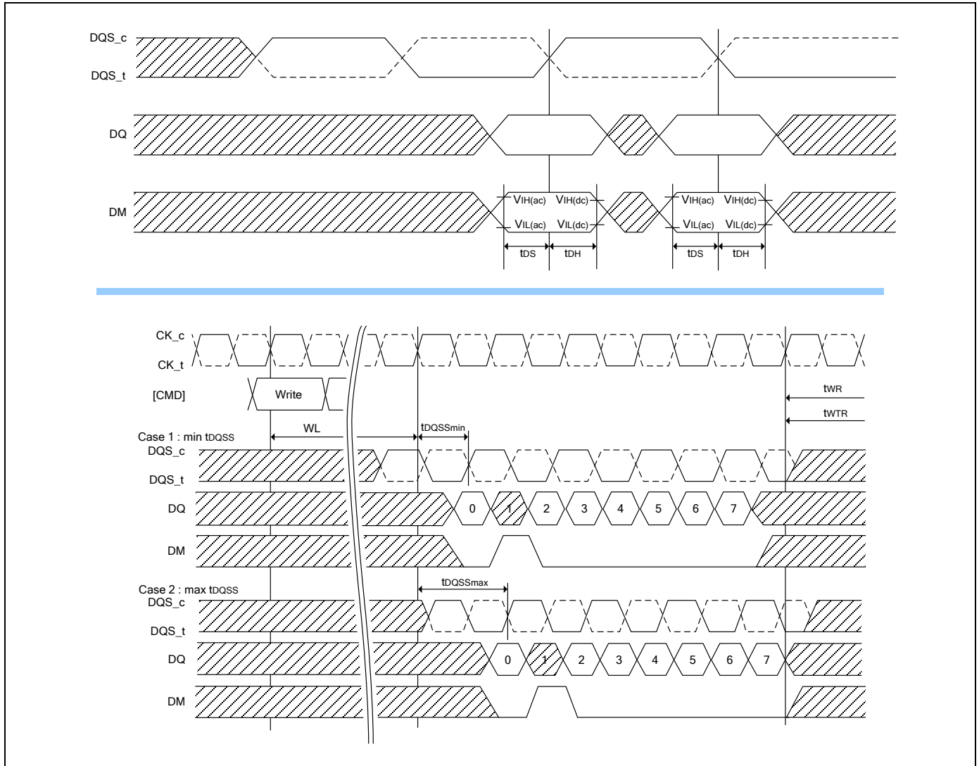
Figure 21 - Data Mask Timing
