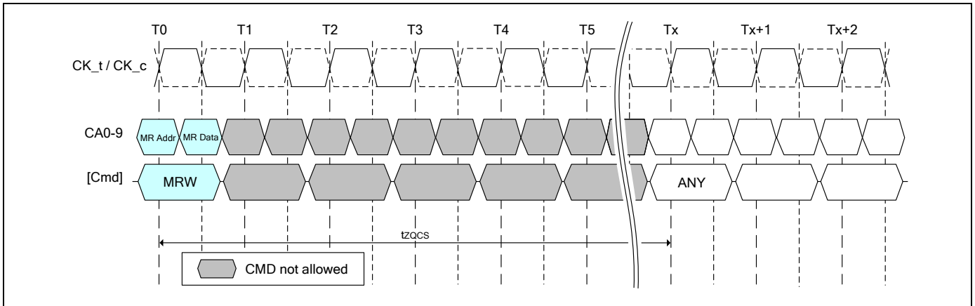
Figure 40 - ZQ Calibration Short Timing
