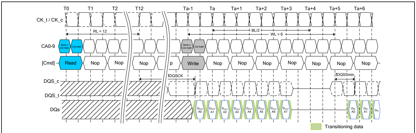
Figure 13 - Burst Read Followed By Burst Write
