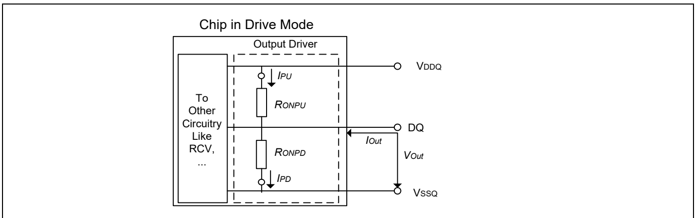
Figure 72 - Output Driver Definition of Voltages and Currents
