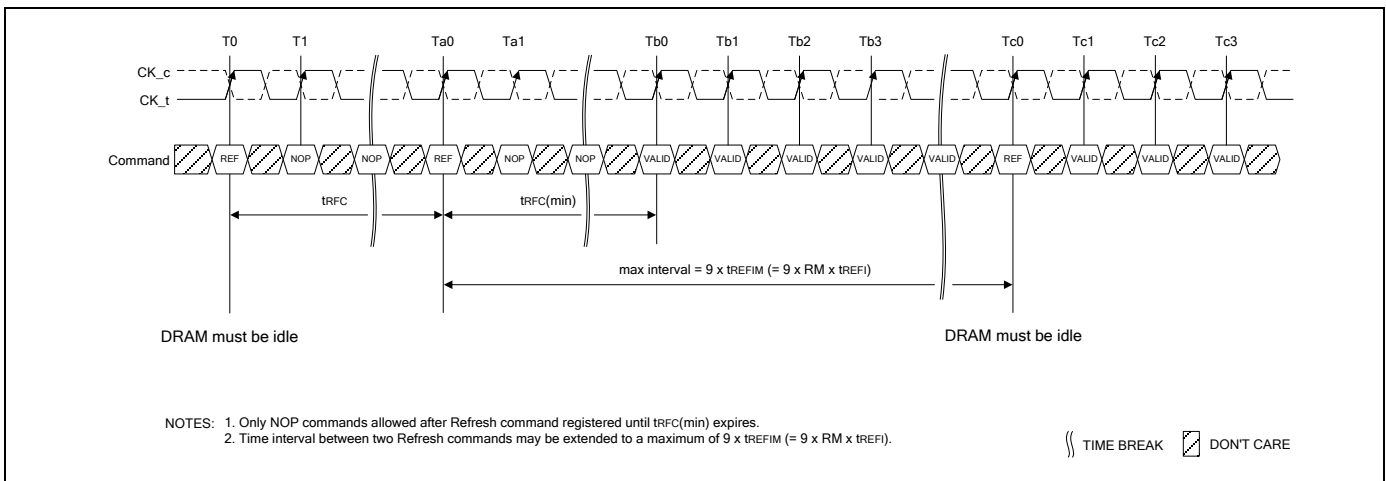
Figure 26 - Refresh Command Timing
