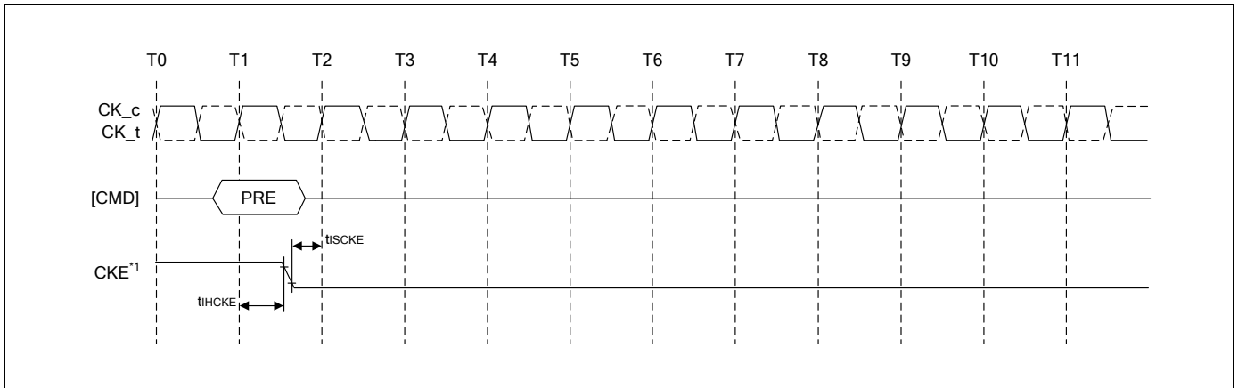
Figure 58 - Precharge Command to Power-Down Entry
