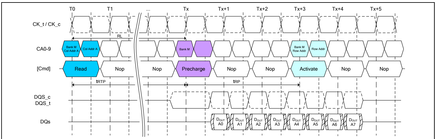
Figure 22 - Burst Read Followed by Precharge
