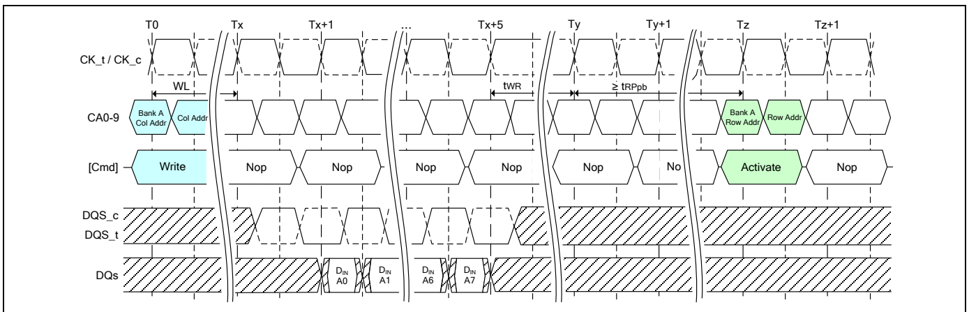
Figure 25 - Burst Write with Auto Precharge
