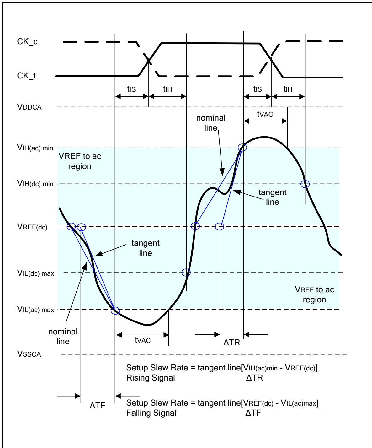
Figure 78 - Tangent line for setup time t IS for CA and CS n with respect to clock
