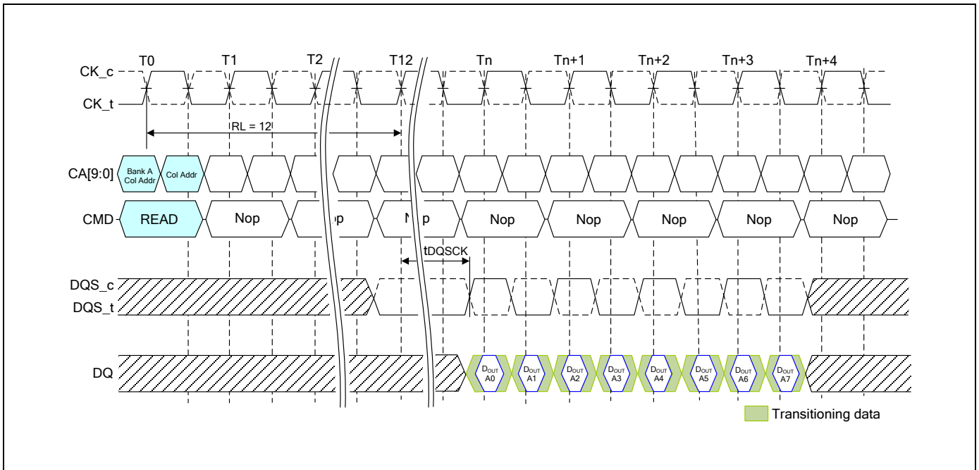
Figure 9 - Burst Read: RL = 12, BL = 8, t_{DQSK} < t_{CK}
