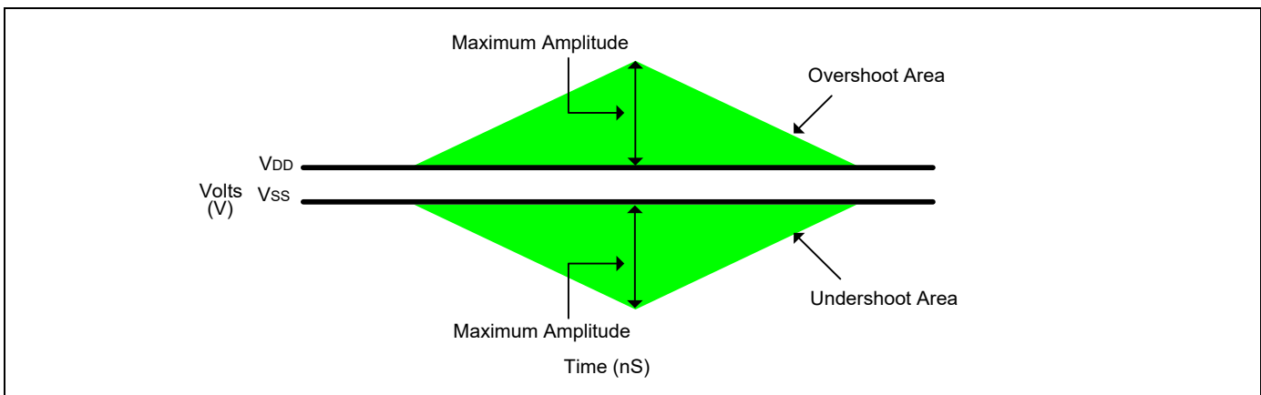
Figure 70 - Overshoot and Undershoot Definition
