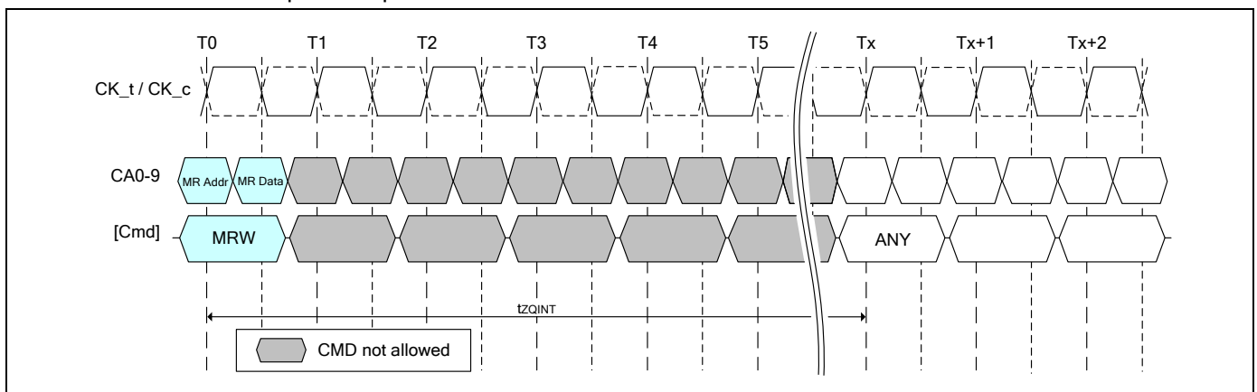
Figure 39 - ZQ Initialization Timing
