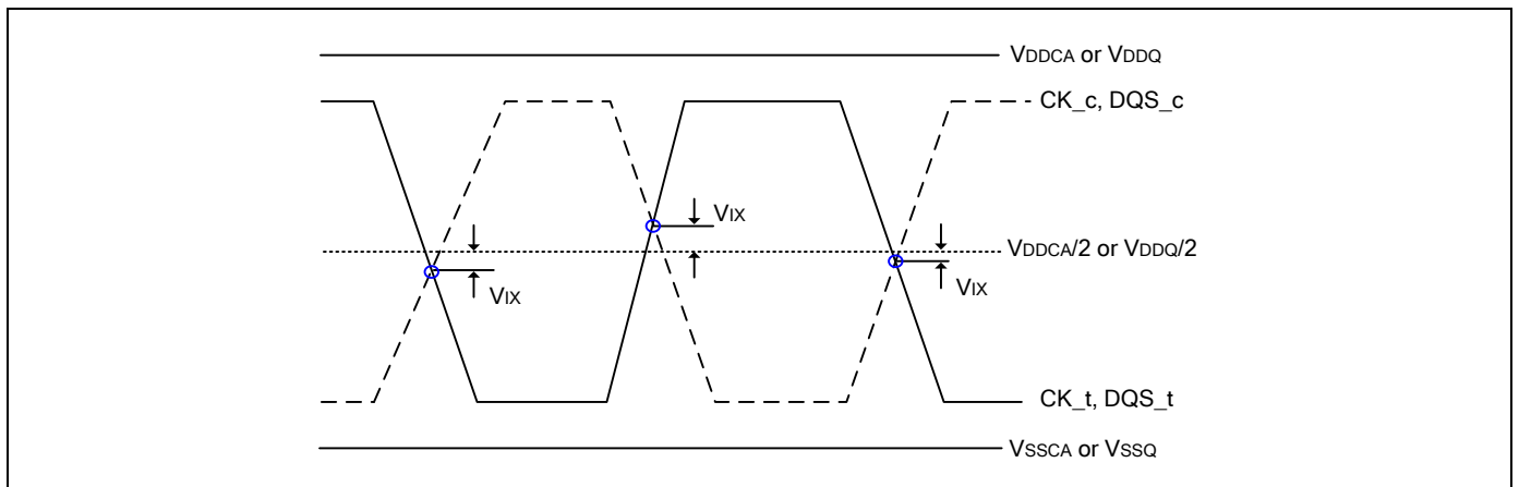
Figure 66 - Vix Definition
