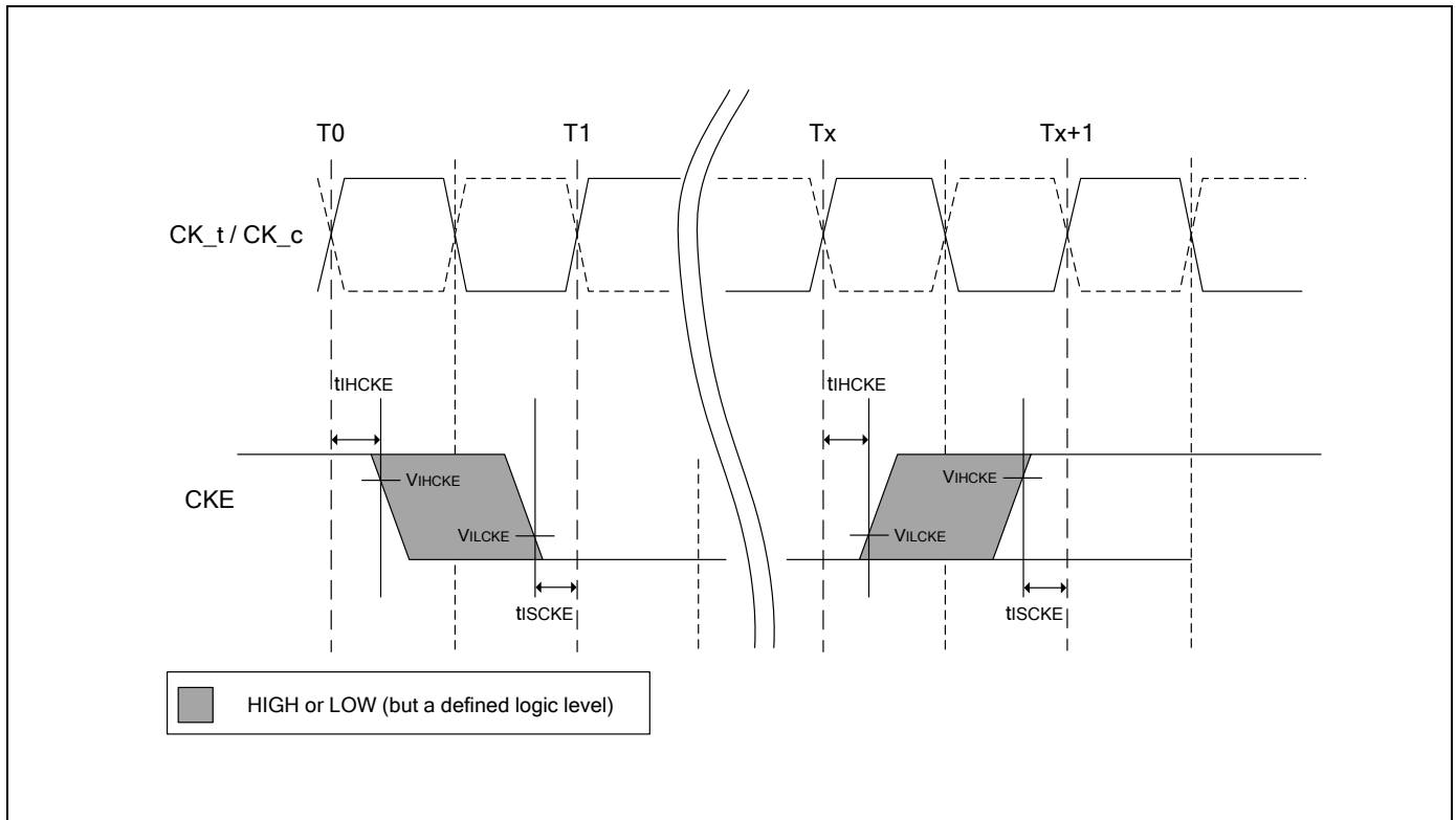
Figure 6 - CKE Input Setup and Hold Timing
