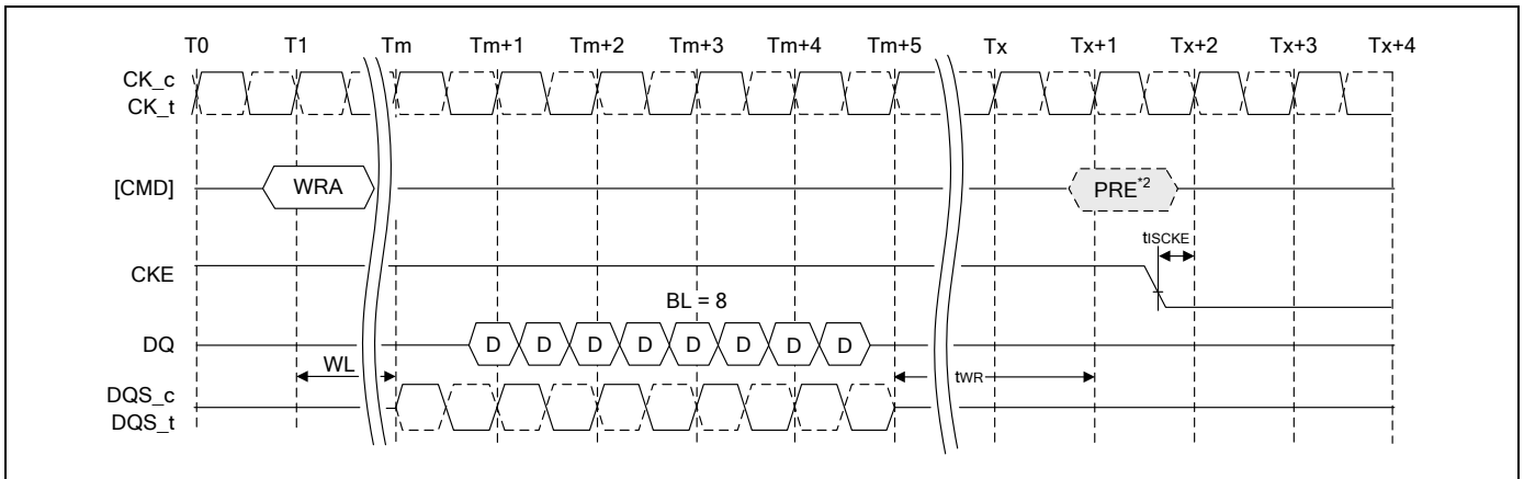
Figure 55 - Write with Auto Precharge to Power-Down Entry
