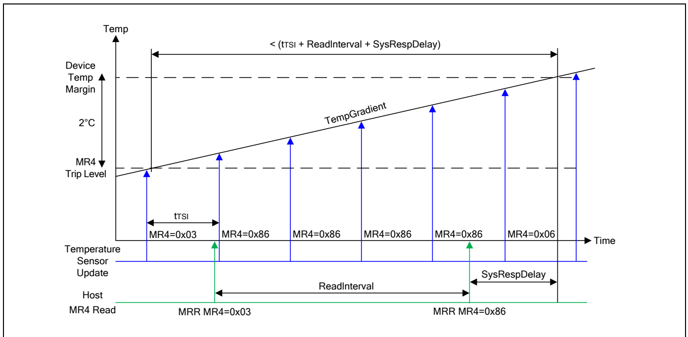
Figure 35 - Temperature Sensor Timing
