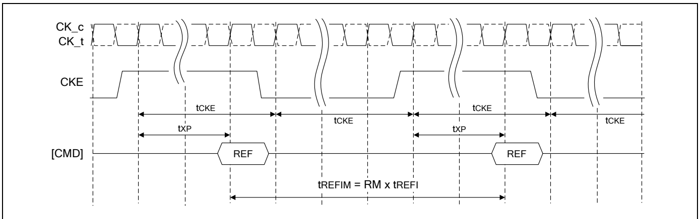
Figure 51 - Refresh-to-Refresh Timing in CKE-Intensive Environments
