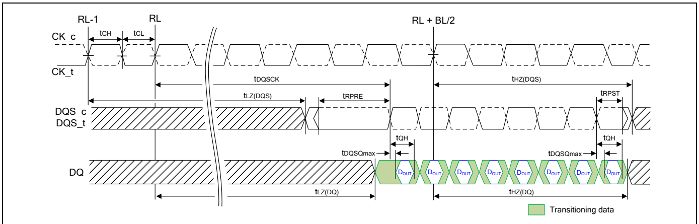
Figure 7 - Read Output Timing
