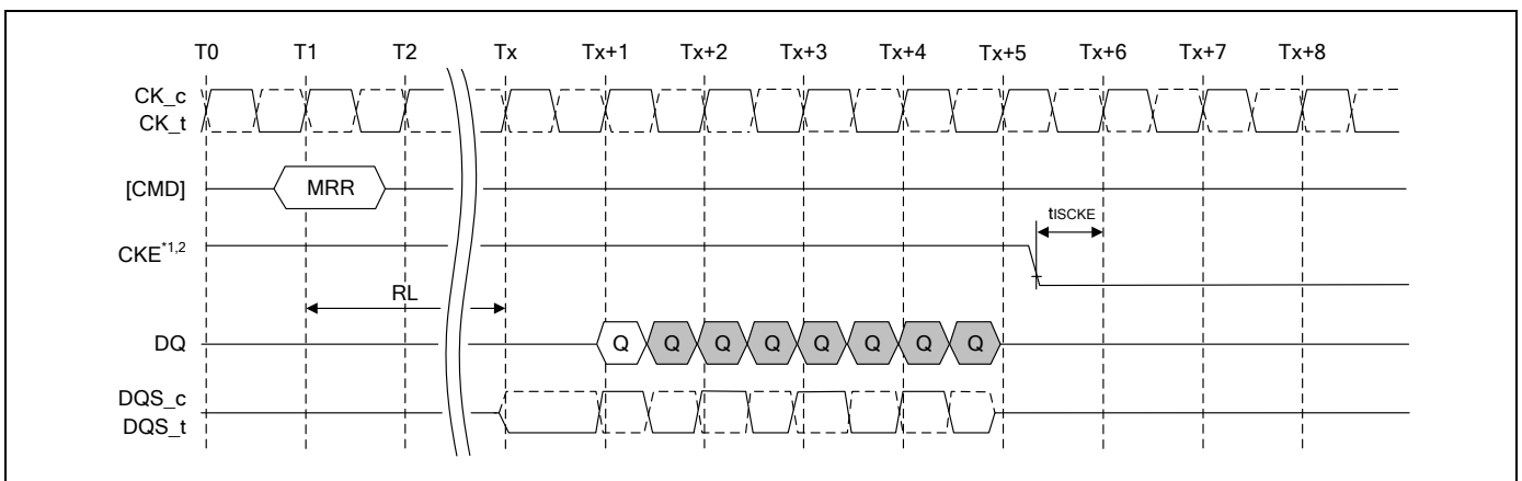
Figure 59 - MRR to Power-Down Entry
