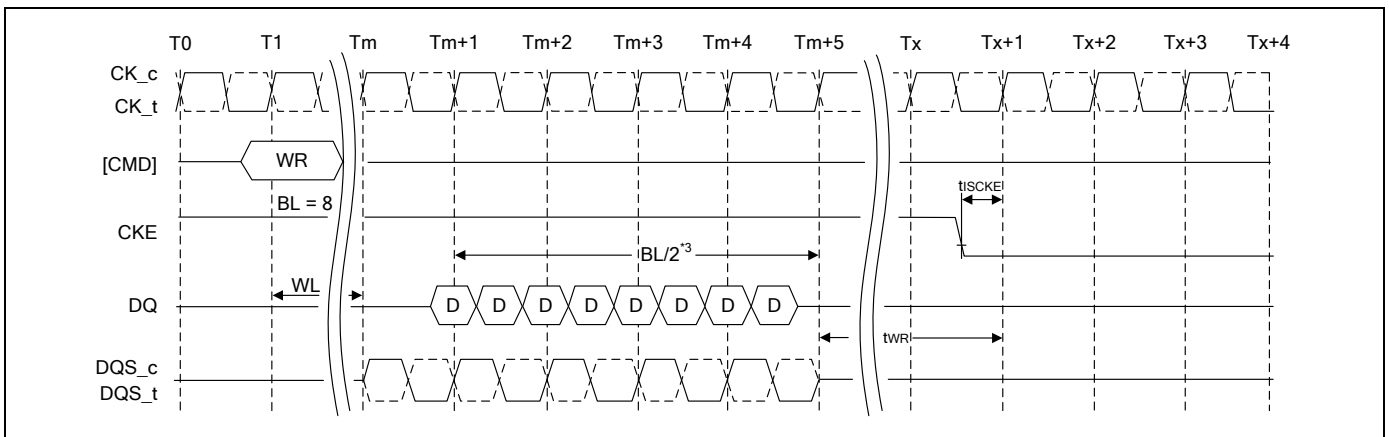
Figure 54 - Write to Power-Down Entry
