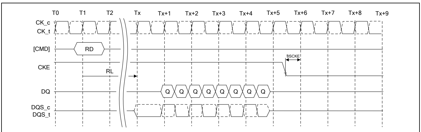
Figure 52 - Read to Power-Down Entry
