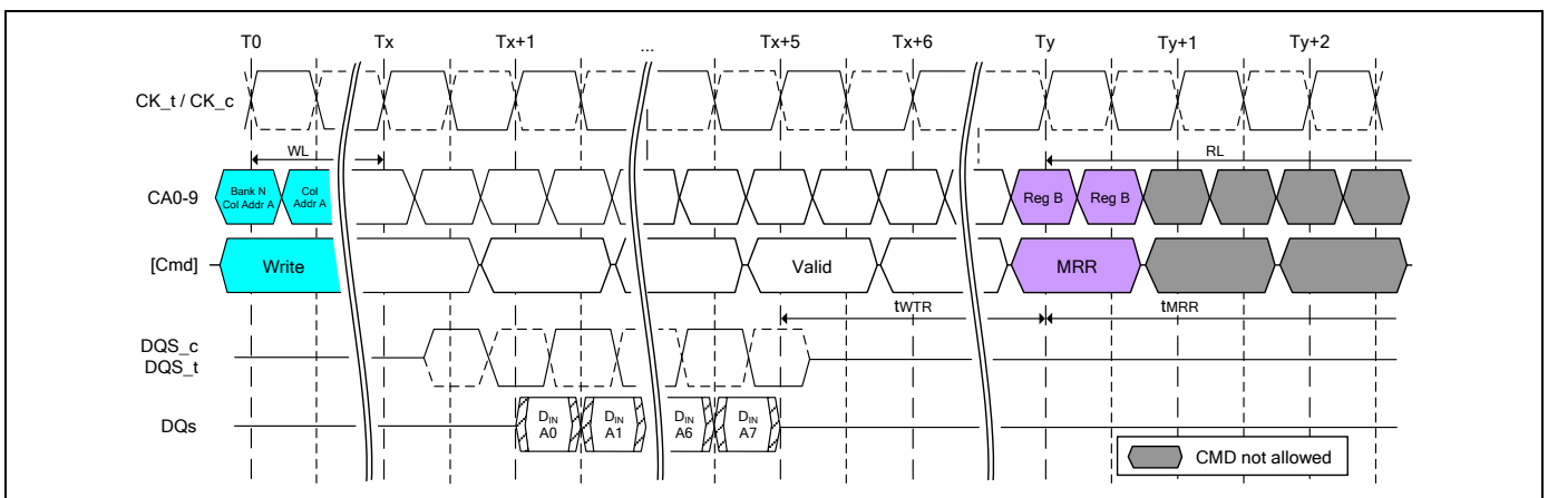
Figure 33 - Burst Write Followed by MRR
