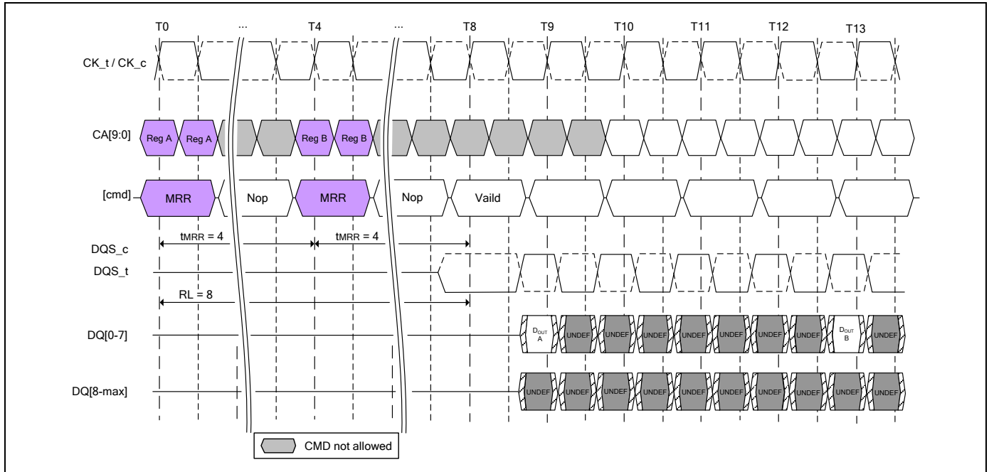
Figure 31 - Mode Register Read timing example: RL = 8
