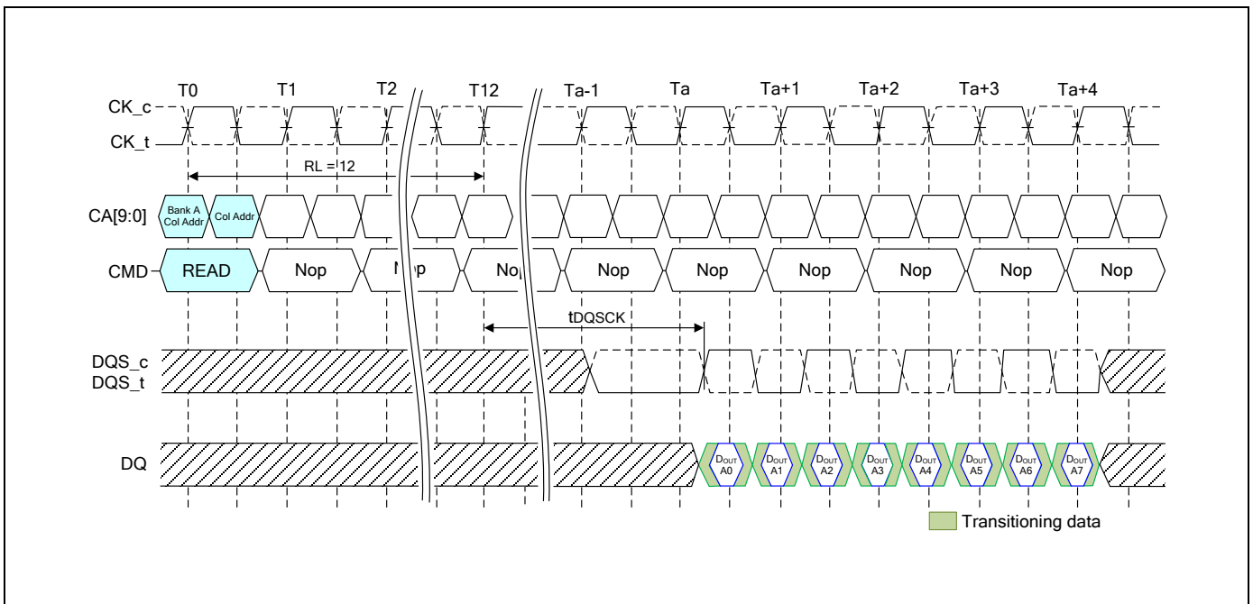
Figure 8 - Burst Read: RL = 12, BL = 8, tDQSCK > tck
