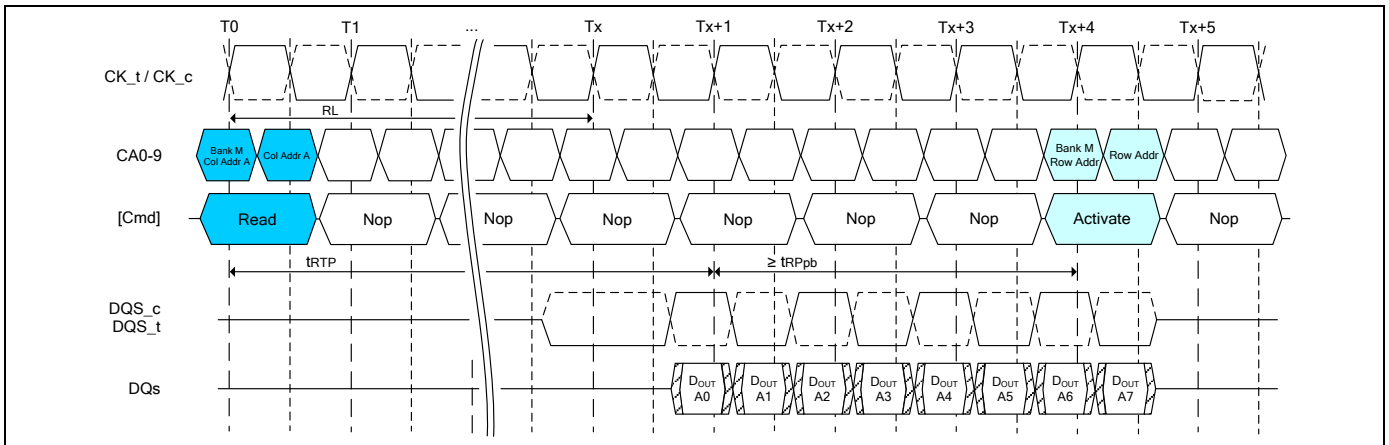
Figure 24 - Burst Read with Auto Precharge
