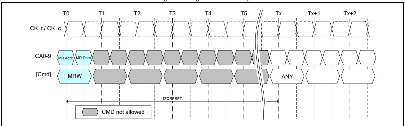
Figure 42 - ZQ Calibration Reset Timing
