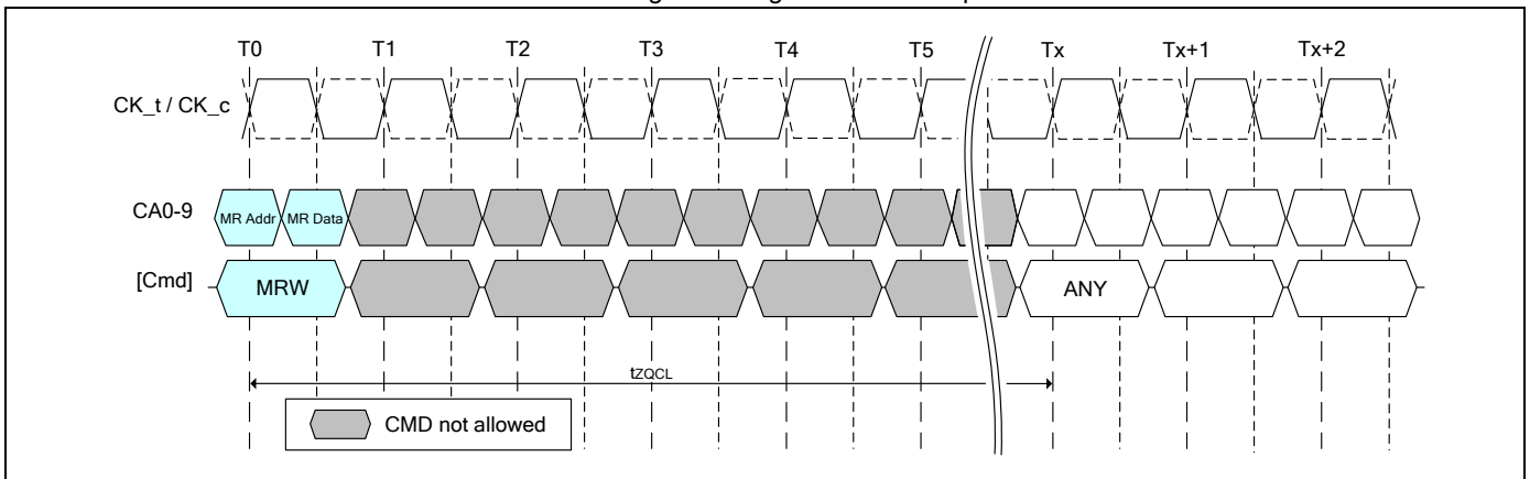
Figure 41 - ZQ Calibration Long Timing
