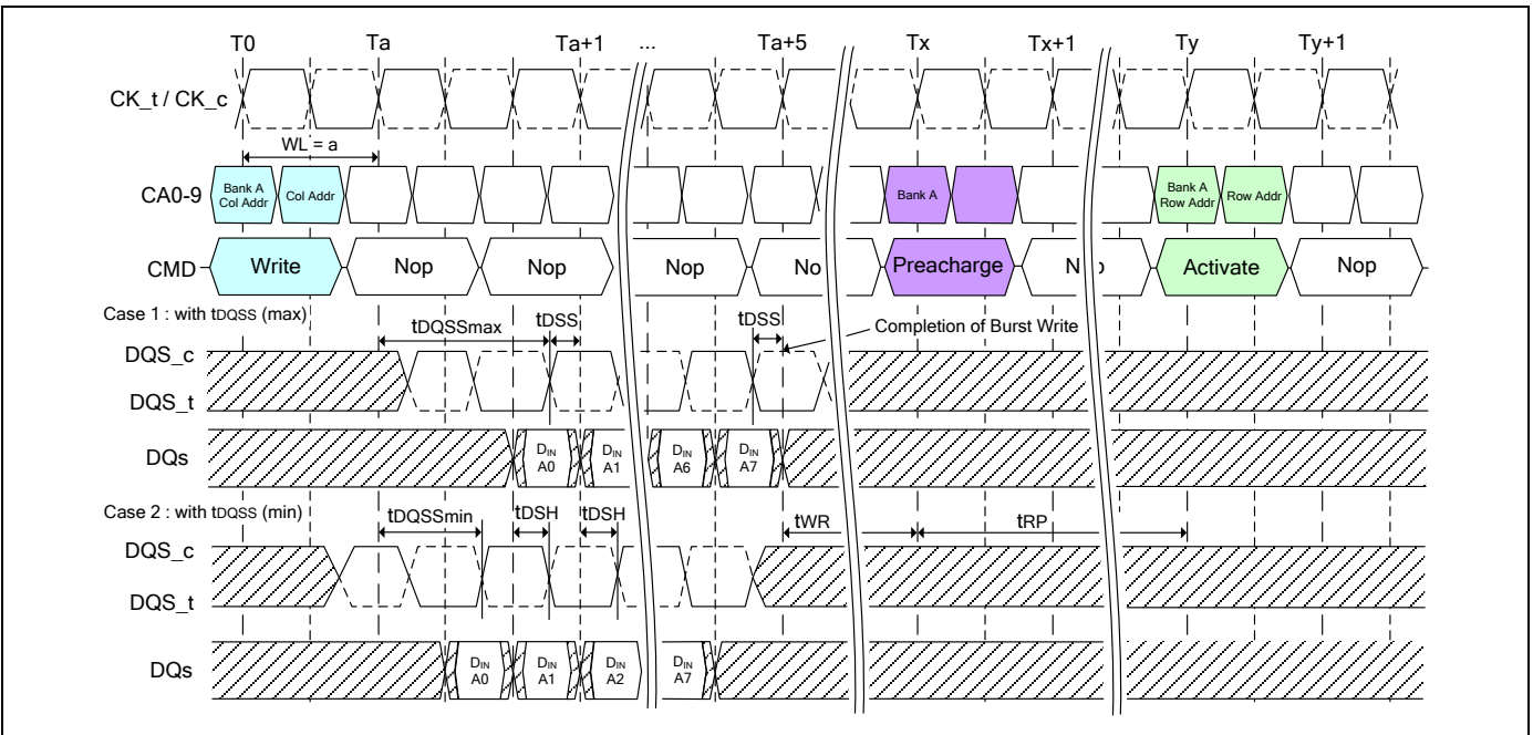
Figure 16 - Burst Write
