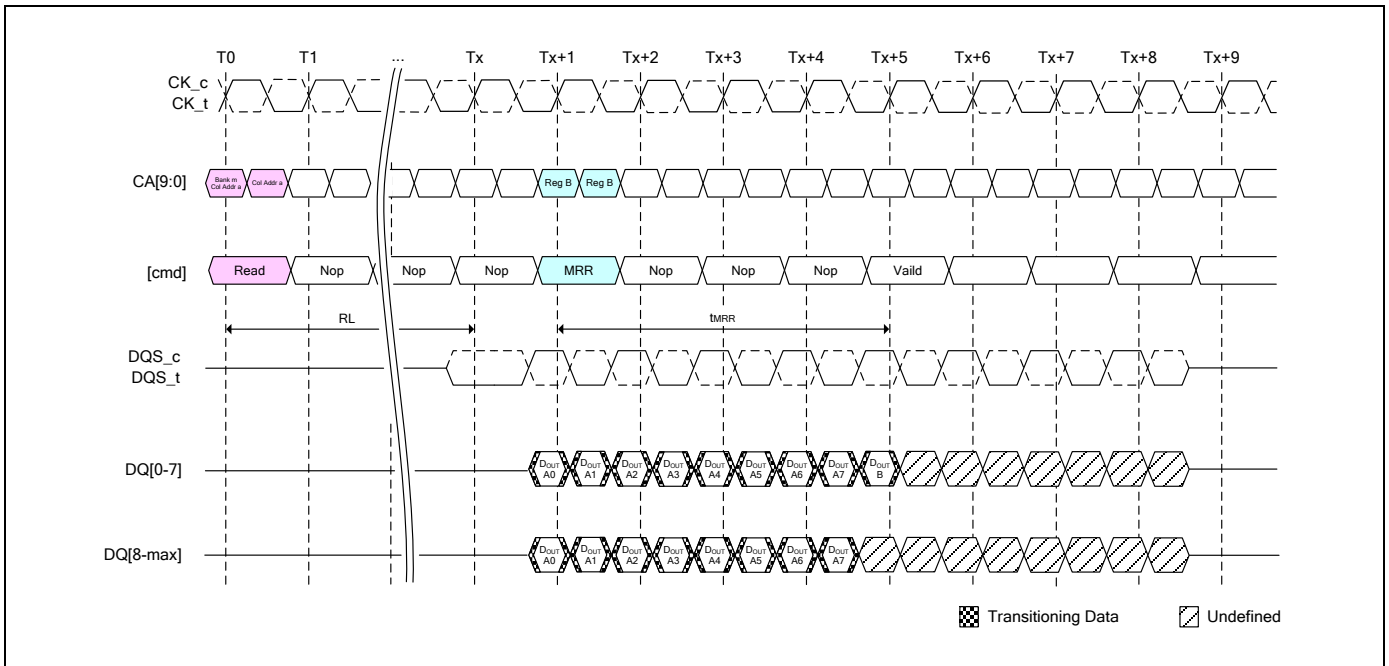
Figure 32 - Read to MRR Timing
