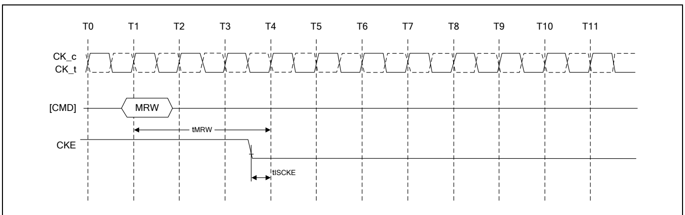
Figure 60 - MRW to Power-Down Entry
