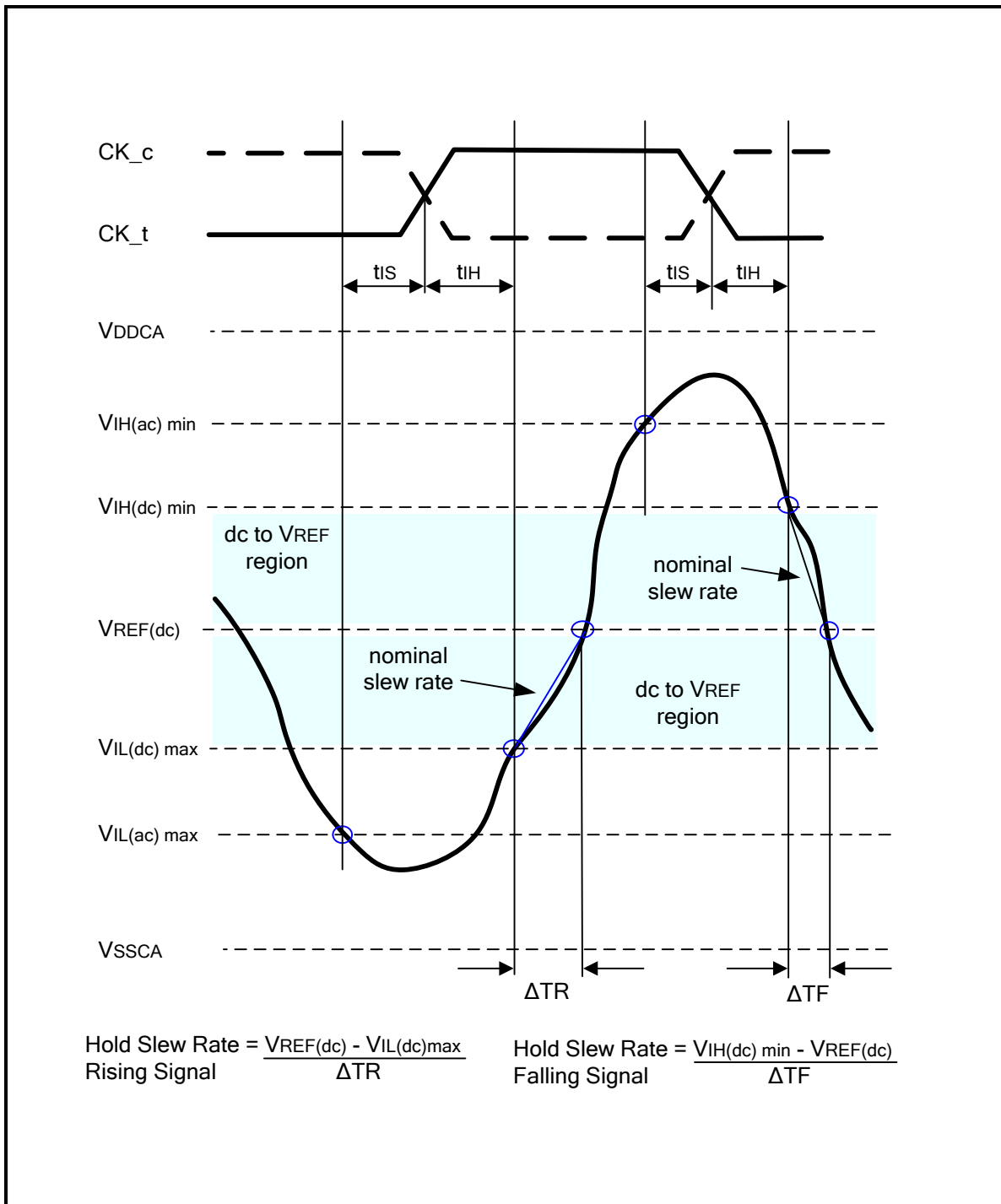
Figure 77 - Nominal slew rate for hold time t_{IH} for CA and CS_n with respect to clock
