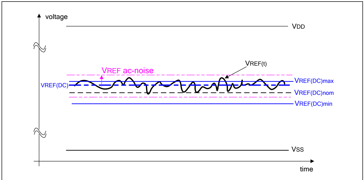
Figure 62 - Illustration of VREF(DC) tolerance and VREF ac-noise limits
