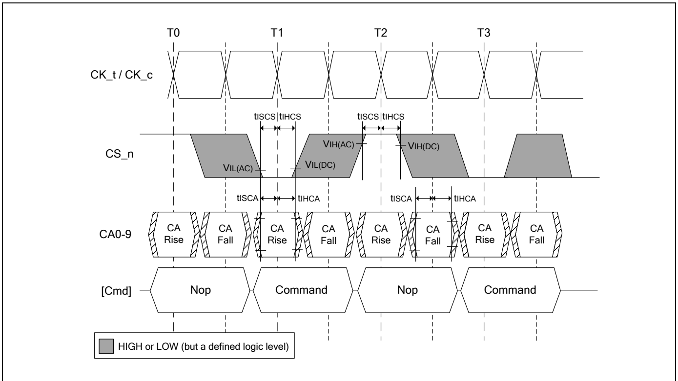
Figure 5 - Command Input Setup and Hold Timing
