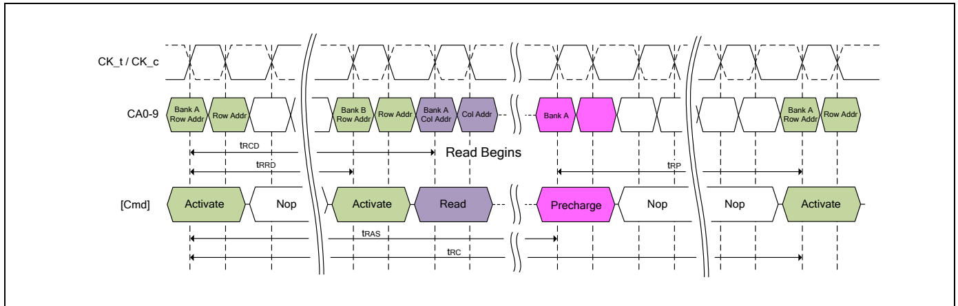
Figure 3 - Activate Command
