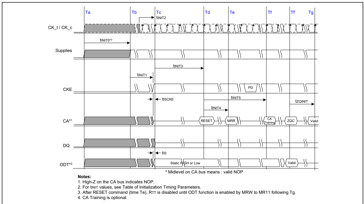
Figure 2 - Voltage Ramp and Initialization Sequence
