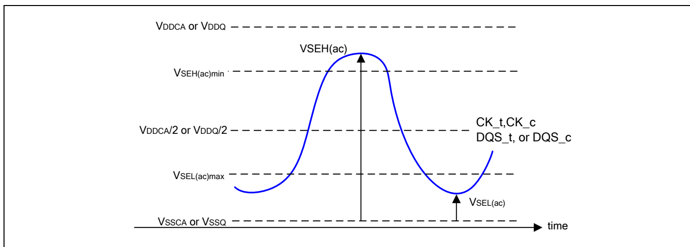
Figure 65 - Single-Ended Requirement for Differential Signals
