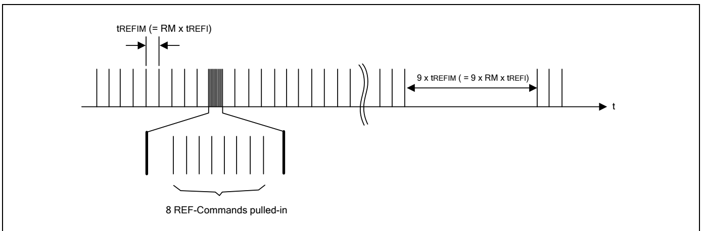
Figure 28 - Pulling-in Refresh Commands
