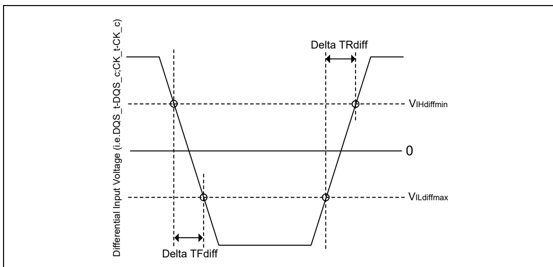
Figure 67 - Differential Input Slew Rate Definition for DQS_t, DQS_c and CK_t, CK_c
